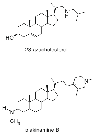
Figure 2. Structures of the cholestan-derived 24-SMT inhibitor and plakinamine B.
